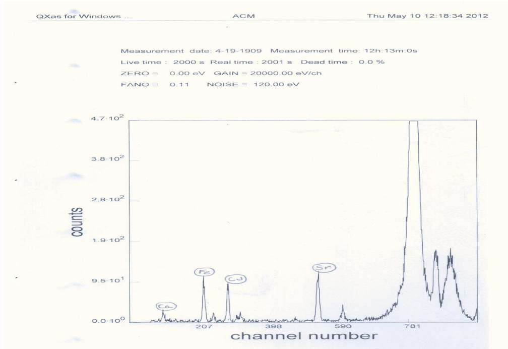
Fig(1). XRF for activated carbon prepared from Mesquite tree ACM
