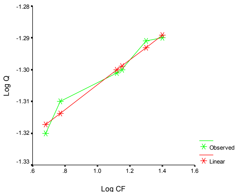
Fig(7). Freundlich isotherm for the adsorption of Cr 3+ on to ACM
