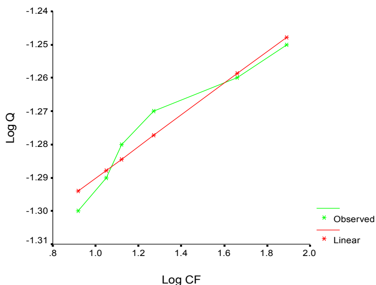
Fig(8). Freundlich isotherm for the adsorption of Co 2+ on to ACM
